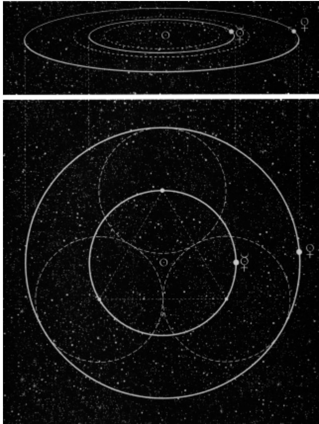
Fig. 19 : John Martineau's illustration of triangular relationship between orbits of Mercury and Venus
