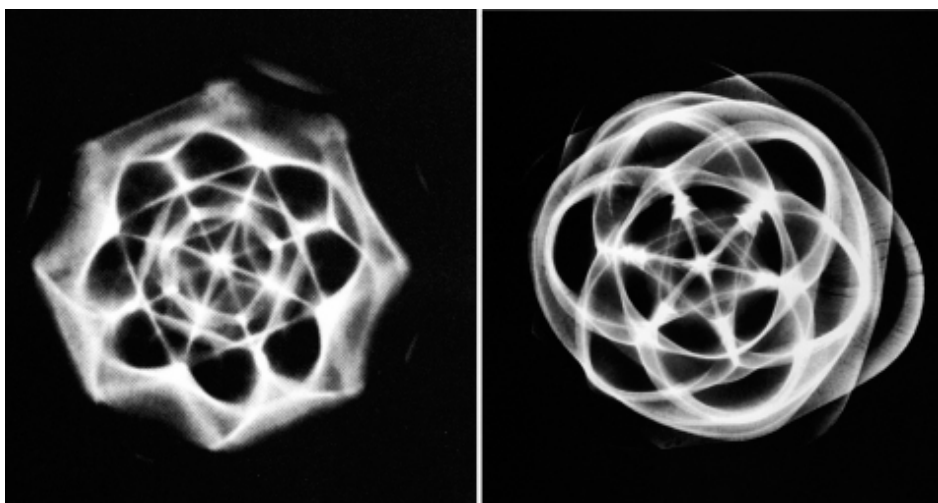
Fig. 21 : Dr. Hans Jenny's illustration of geometry in a vibrating fluid. Sand particles form two different complex shapes as sound frequency changes.
