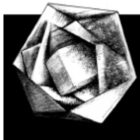
Fig. 22 : Dr. Robert Moon’s geometric model of the atomic nucleus
