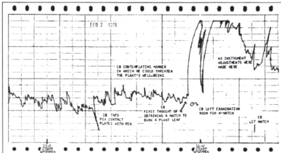
Fig. 6: Dr. Cleve Backster’s diagram of humanlike electrical activity in a plant
