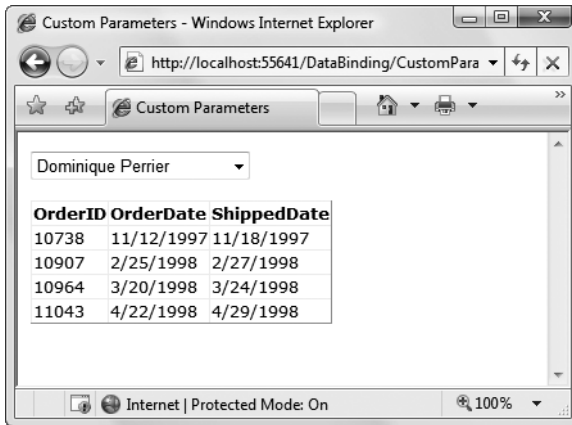
Figure 16-13. Using parameters in a master-details page
