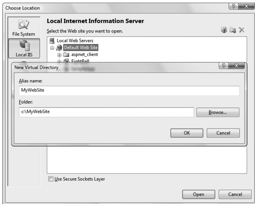
Figure 9-19. Creating a virtual directory in a specific location
