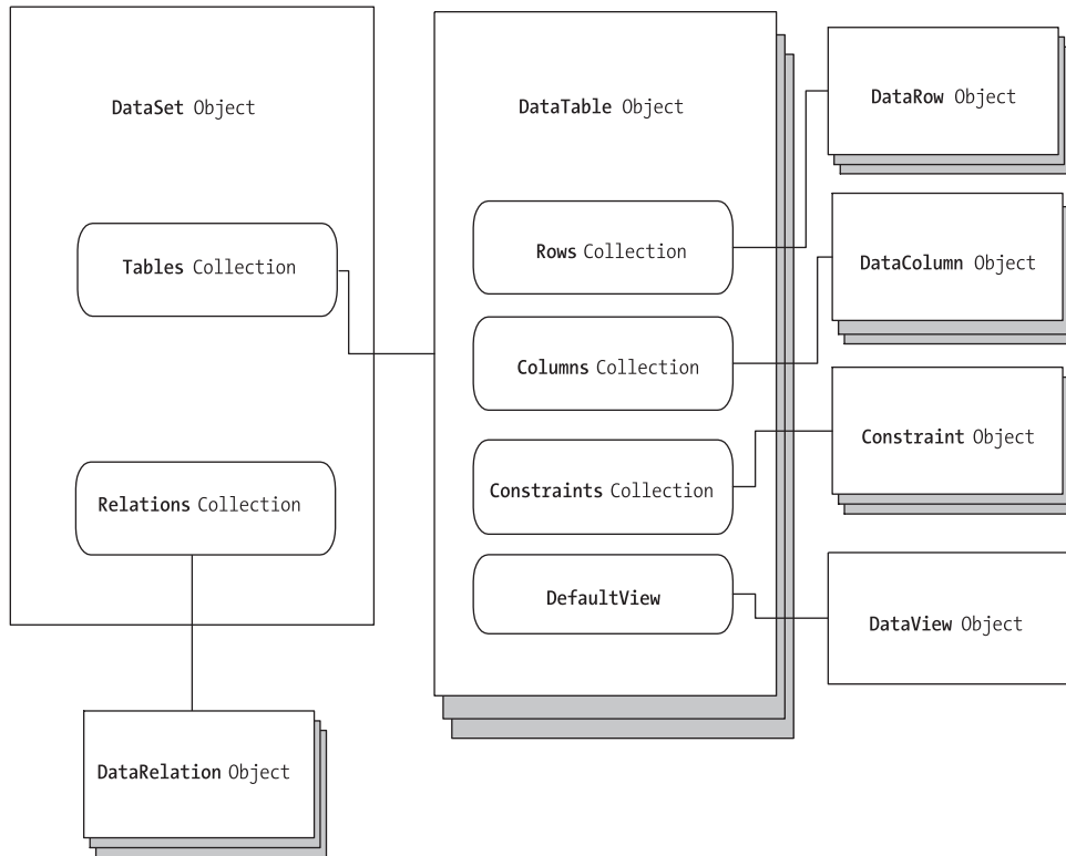
Figure 15-16. The DataSet family of objects
