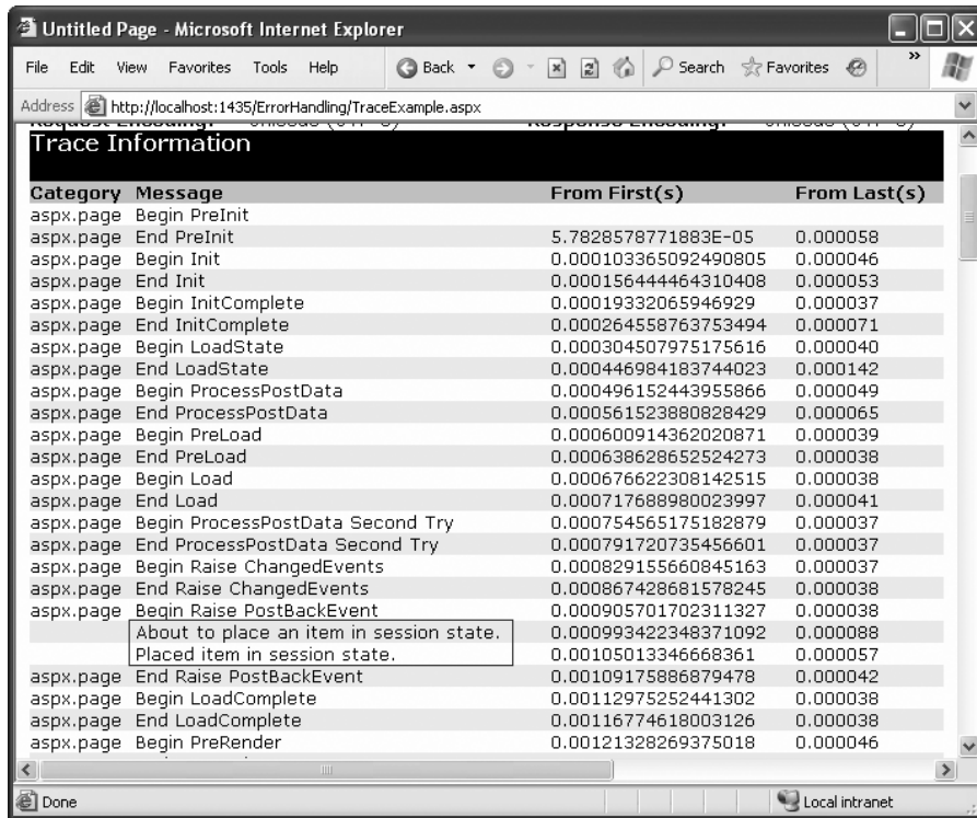
Figure 8-25. Custom trace messages
