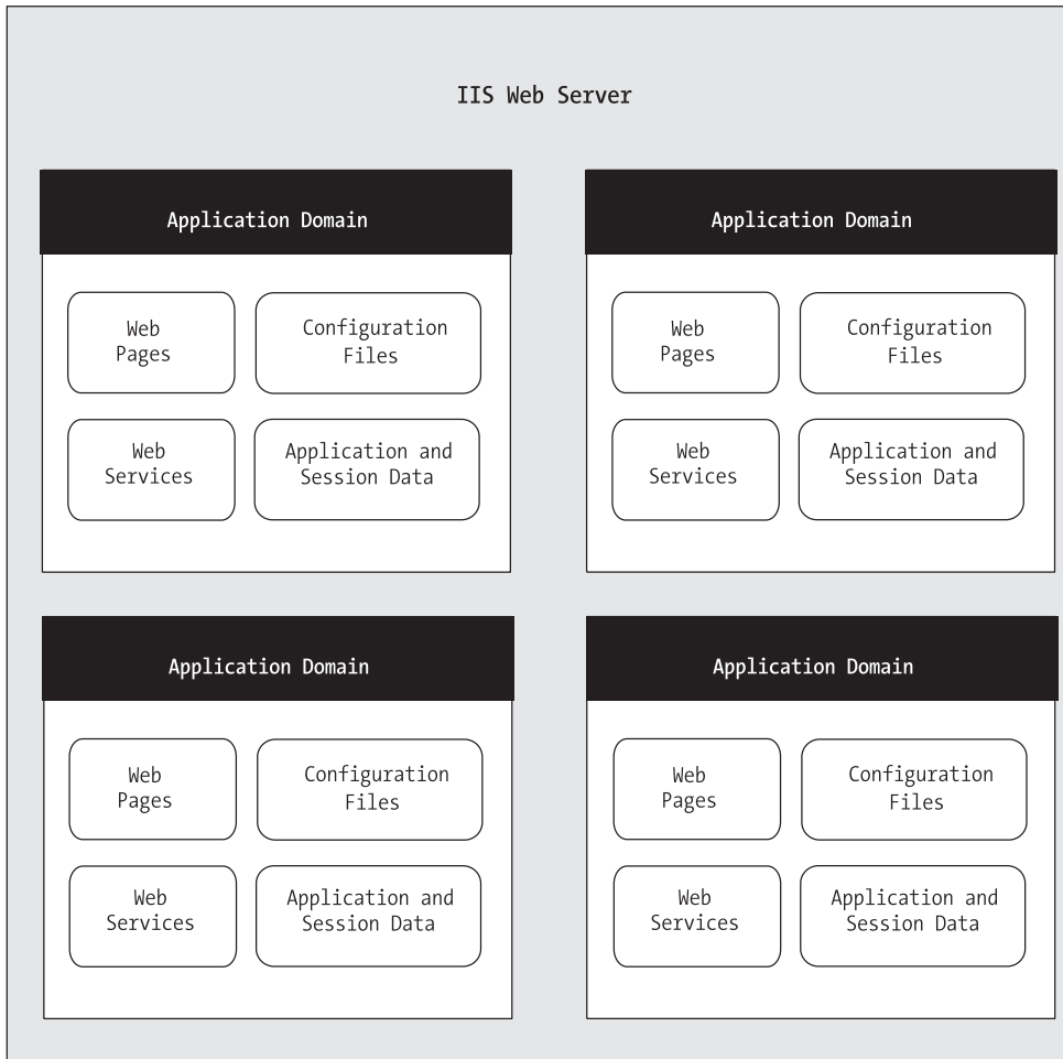
Figure 5-1. ASP.NET applications
