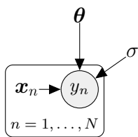
training set Figure 9.3 Probabilistic graphical model for linear regression. Observed random variables are shaded, deterministic/known values are without circles.
